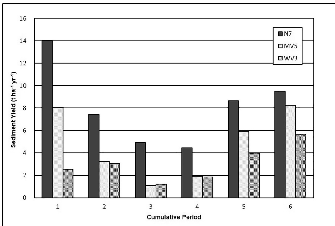
Fig. 13. Sediment yield comparison by site for six cumulative periods. Dark gray is N7 native (undisturbed by mining), light gray is MV5 fluvial geomorphic design with topdressing and poor to moderate vegetation, and medium gray is WV3 fluvial geomorphic design with topdressing and significant vegetation establishment.
