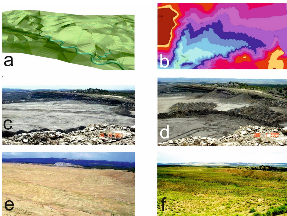
Fig. 5. a) shows a 3D perspective view of an example GeoFluv design, b) is a plan view draft of a highwall reclamation project colored by elevation intervals, c) the early stage of reclamation earthwork to reclaim a highwall, d) the waste earth material is beginning to be placed according to the fluvial geomorphic design to make the reclamation landform, e) earth material has been graded to the fluvial geomorphic design and a suitable topdressing for reseeding applied, and f) shows the completed fluvial geomorphic highwall reclamation on the upper right to center (much of the remaining 15.4 ha subwatershed area is shown on the left).
