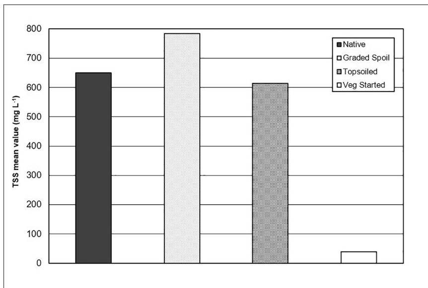
Fig. 3. Average suspended sediment concentration (TSS) in grab samples from native and constructed fluvial geomorphic reclamation on the mine site; October 7, 2007.
