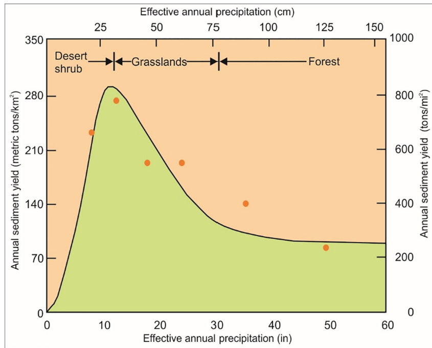
Fig. 2. Graphic representation of the relationship between sediment yield, precipitation, and vegetation type (Langbein and Schumm, 1958). The La Plata Mine study site's 285 mm (11.21 in.) average precipitation value is in the range associated with the maximum erosion and sediment yield.
