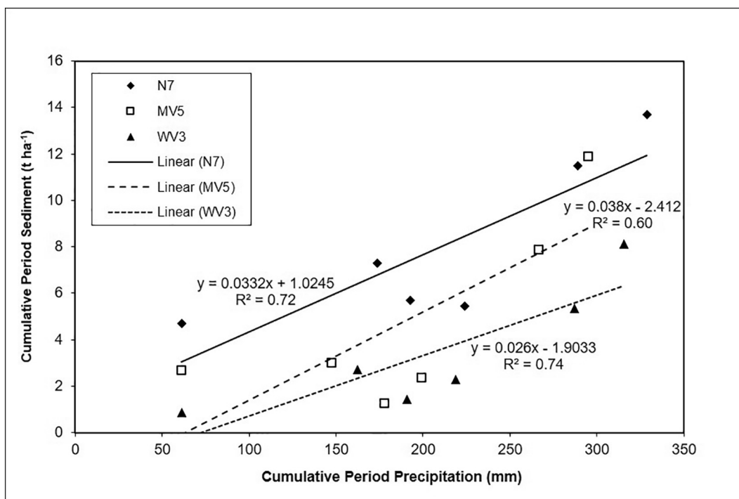
Fig. 14. This cumulative period sediment versus cumulative period precipitation plot shows the linear regression relationships that presented for the three sites.
